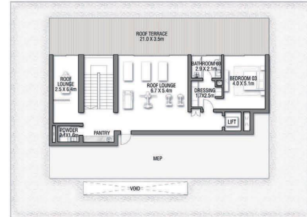
SECOND FLOOR
