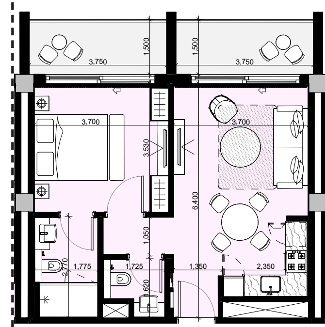
1 BEDROOM TYPE 04 58.74 m 2
