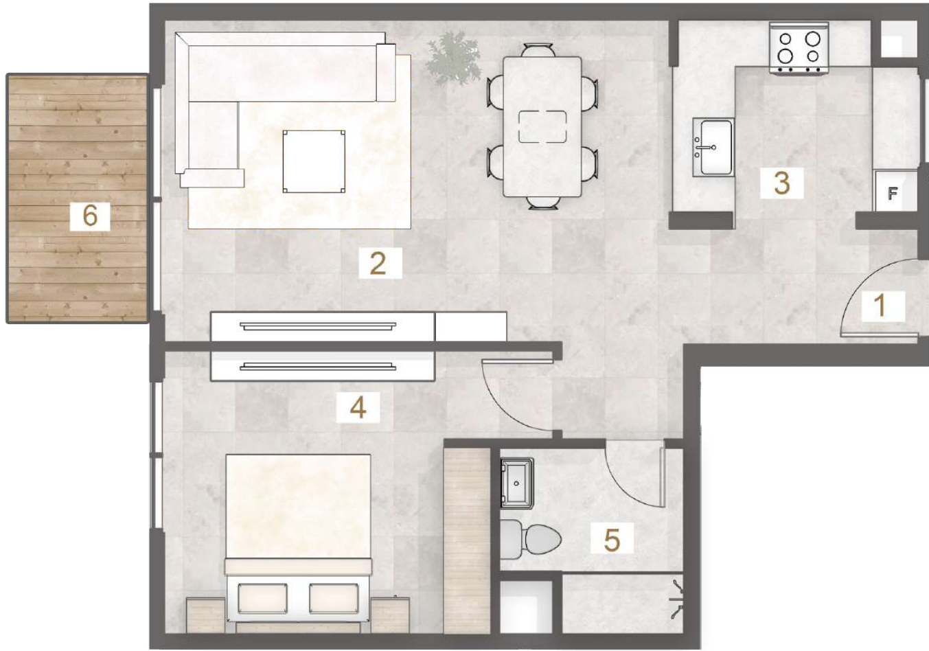
KEY PLAN
