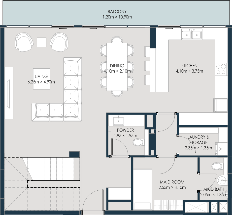
14th Floor
