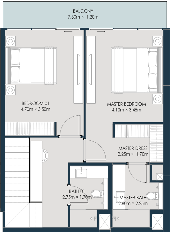
7th Floor
