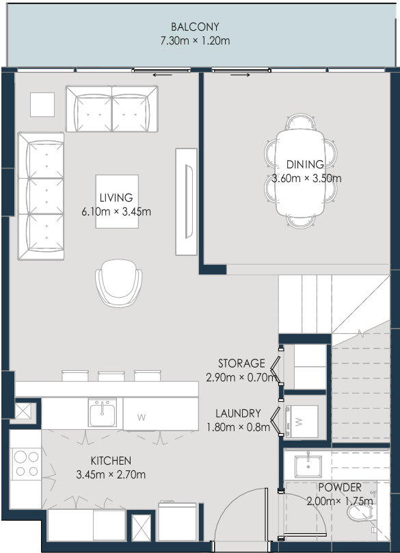
14th Floor
