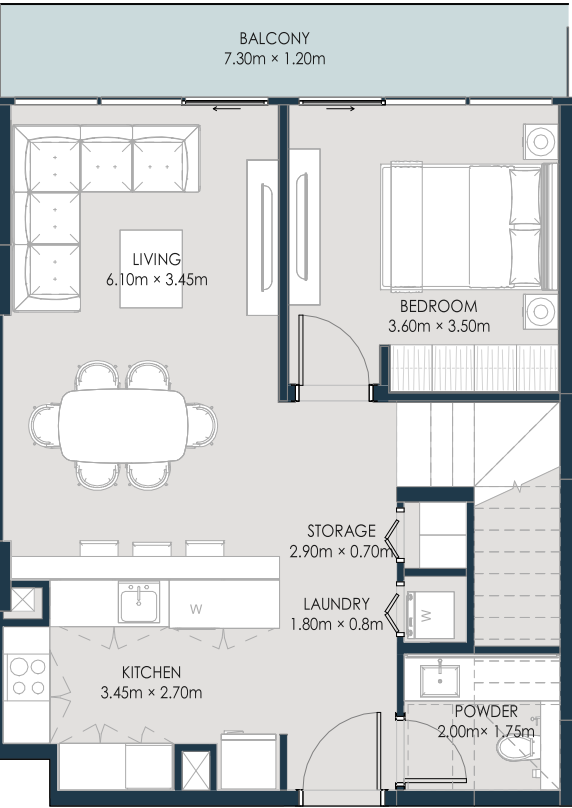
14th Floor
