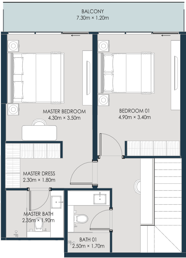
7th Floor
