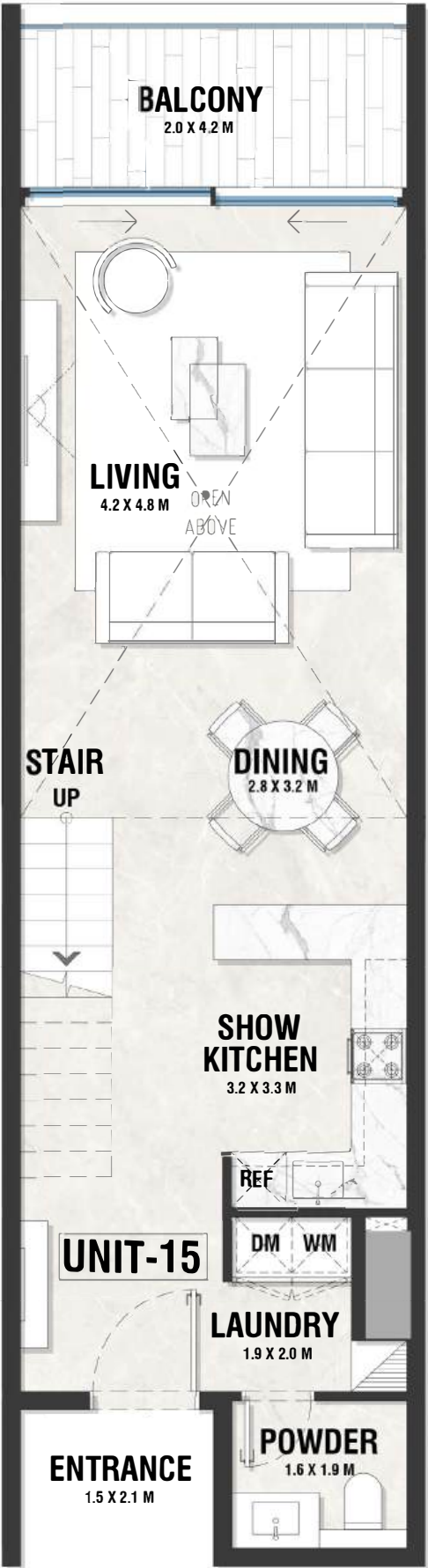
LOWER LEVEL LOFT
