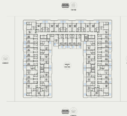
4th Floor Plan Key Plan
