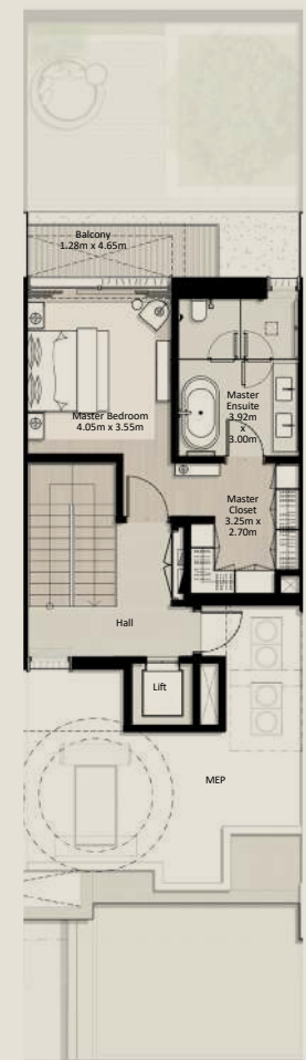
SECOND FLOOR
