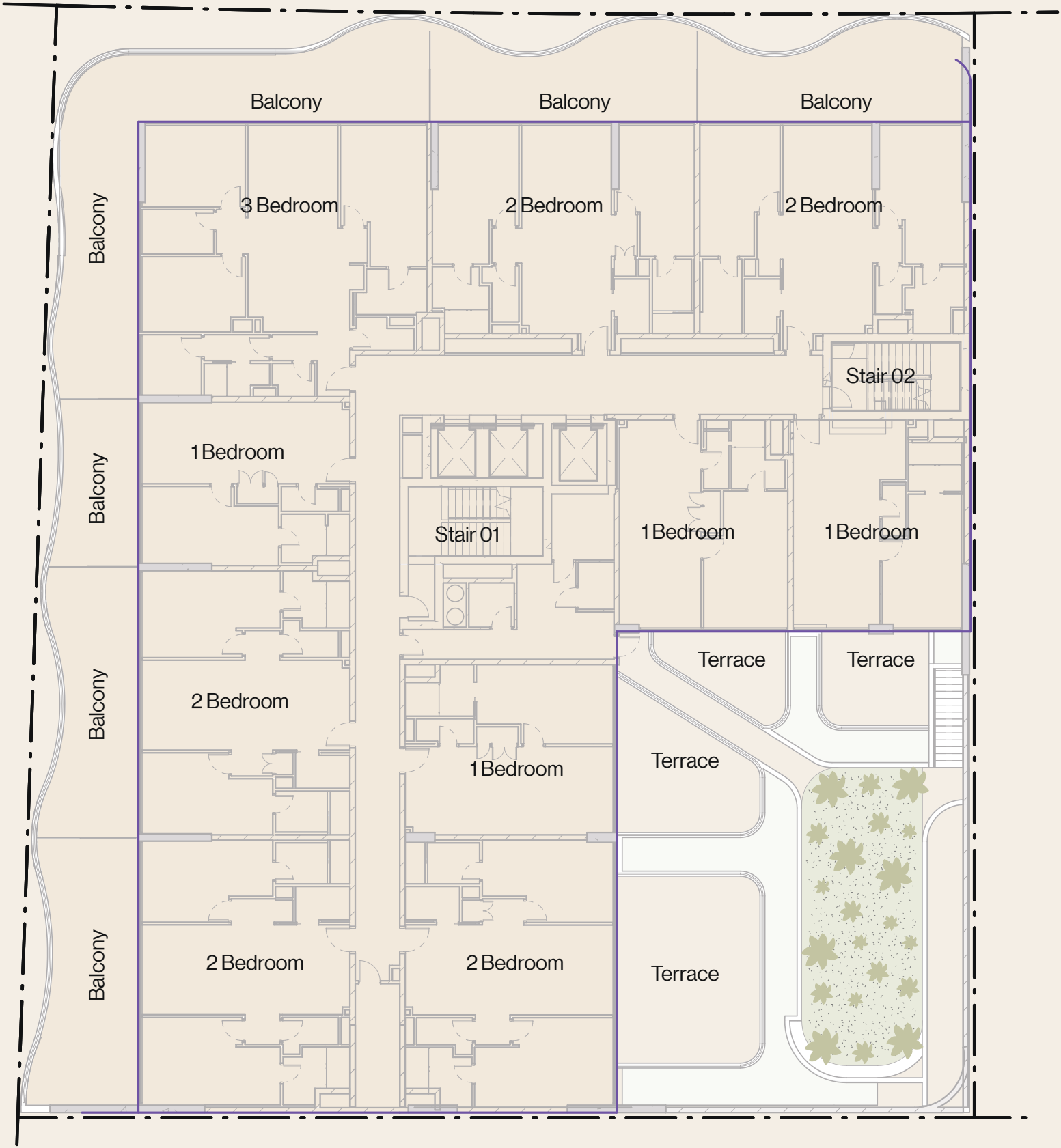
Level 01 floor plate
